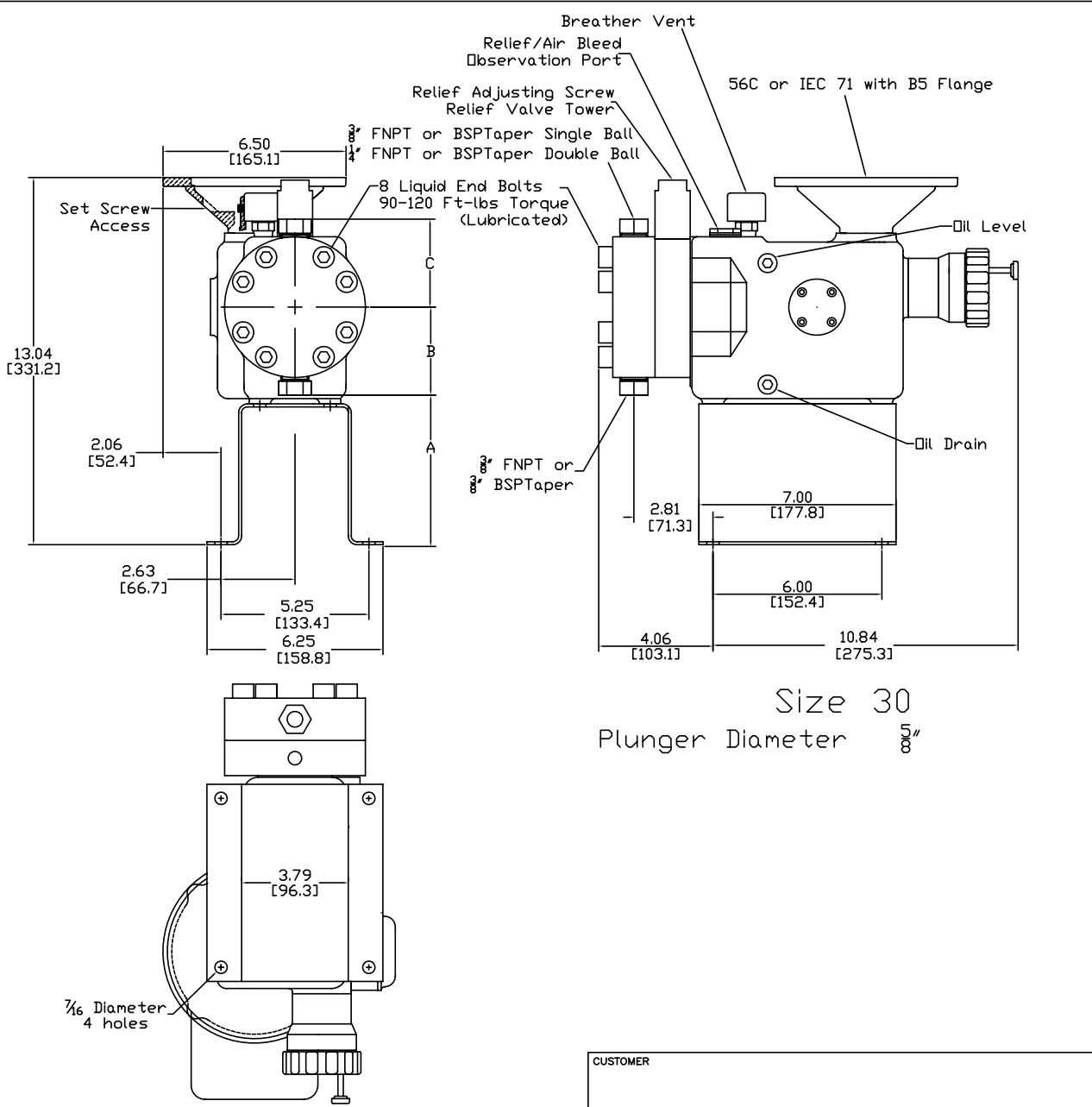
Dimensional Drawing / ProMus Size 30A Metal Liquid End
