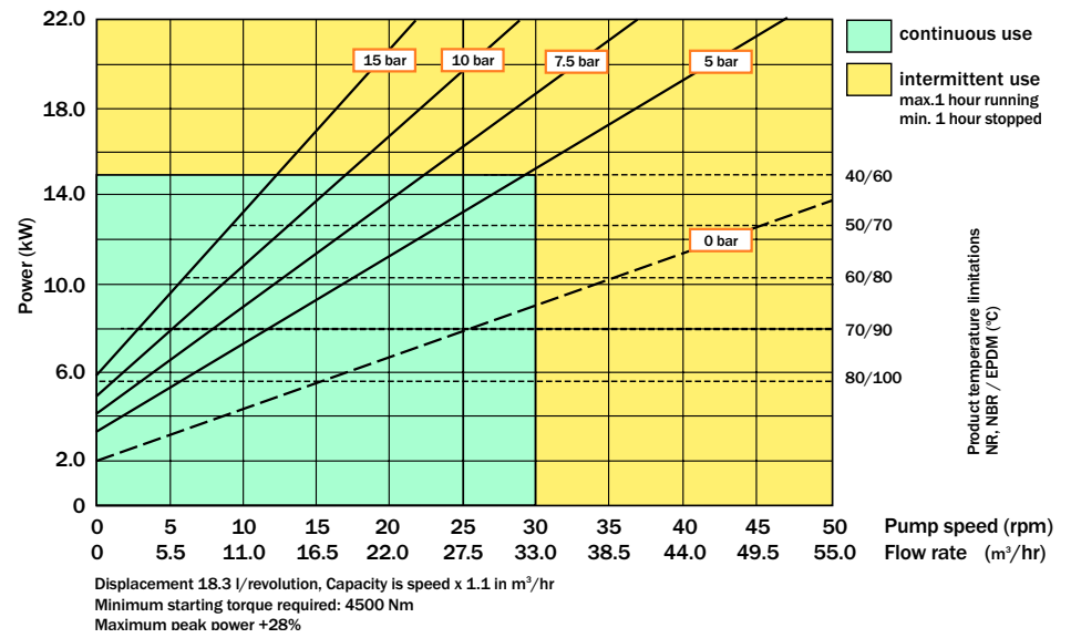
Performance curve VF100
