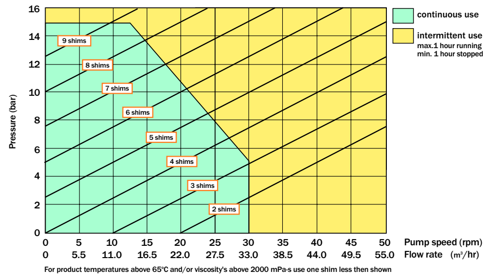
Shimming curve VF100
