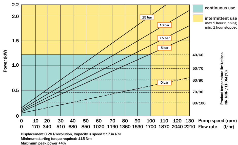
Performance curve VF25
