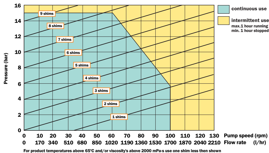
Shimming curve VF25
