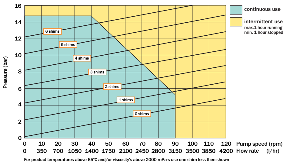
Shimming curve VF32
