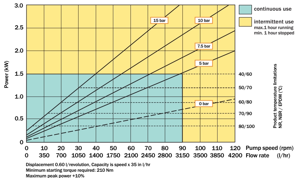
Performance curve VF32
