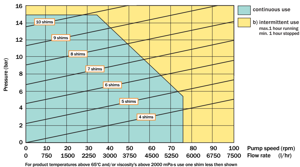
Shimming curve VF40
