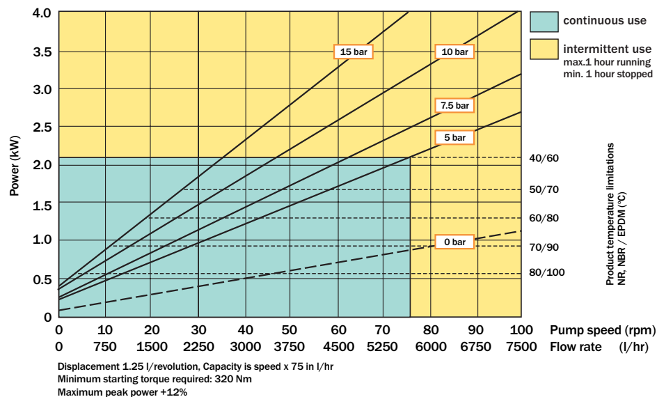
Performance curve VF40
