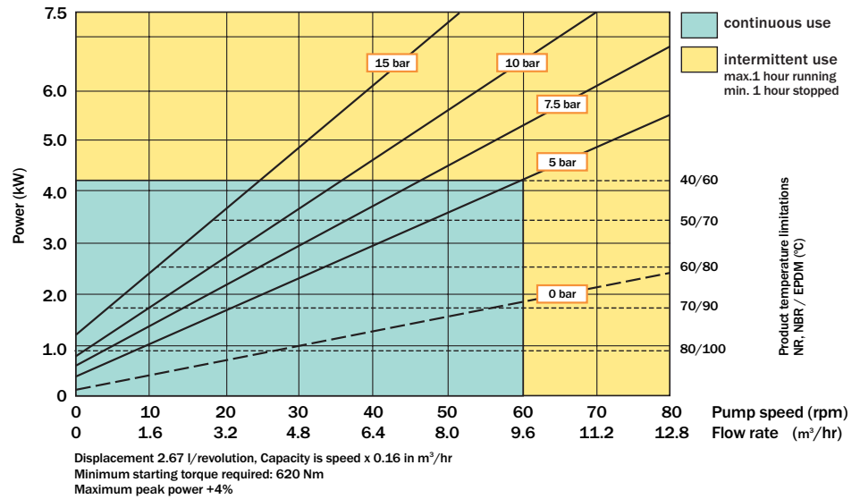
Performance curve VF50
