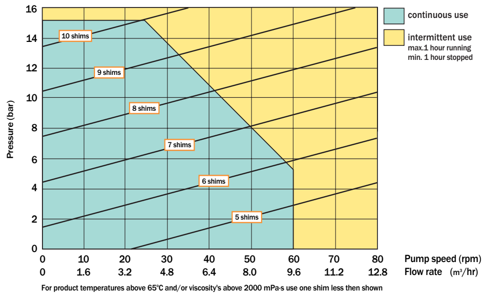
Shimming curve VF50
