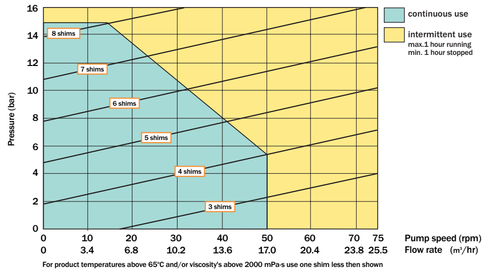
Shimming curve VF65
