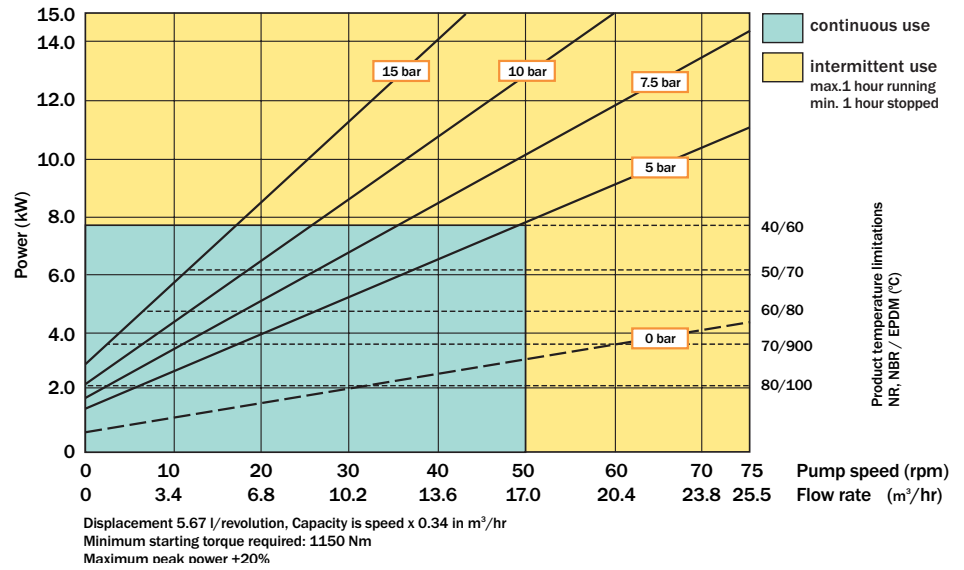
Performance curve VF65
