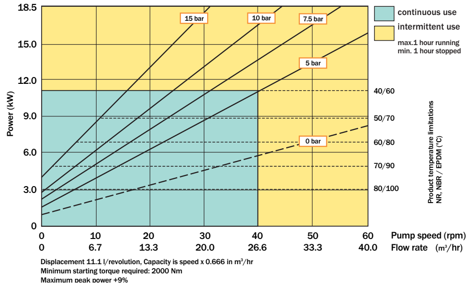
Performance curve VF80
