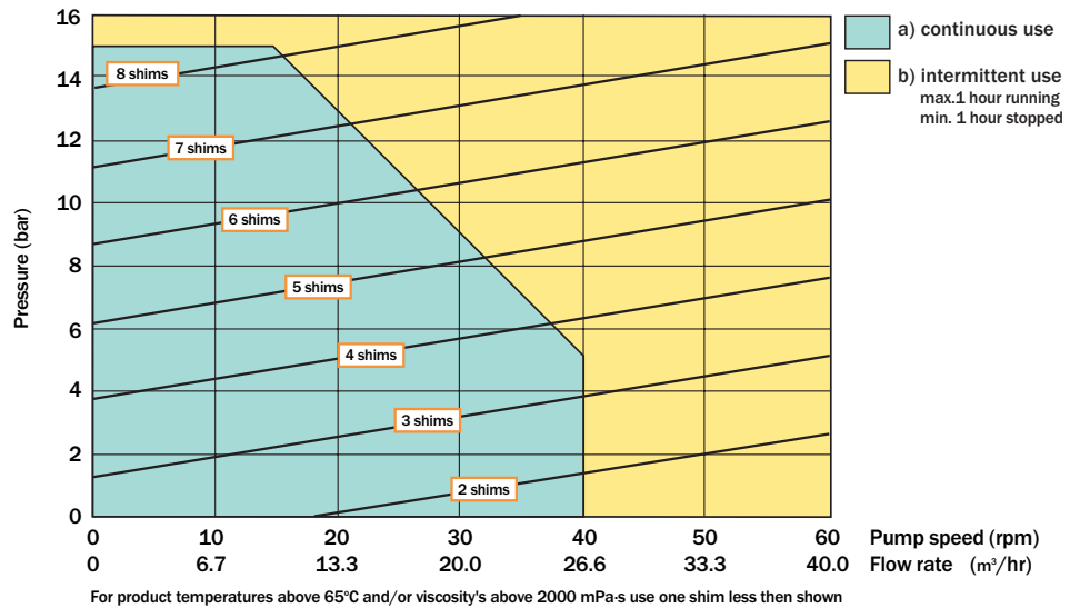
Shimming curve VF80
