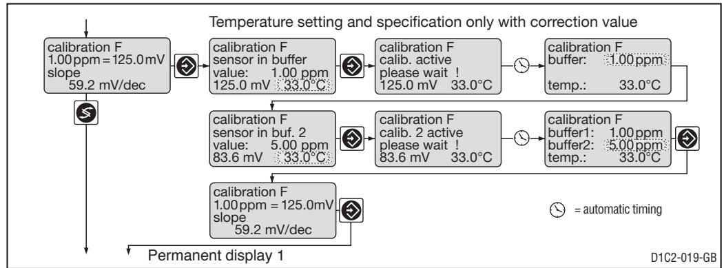
b) Two-point calibration in the full operating menu
